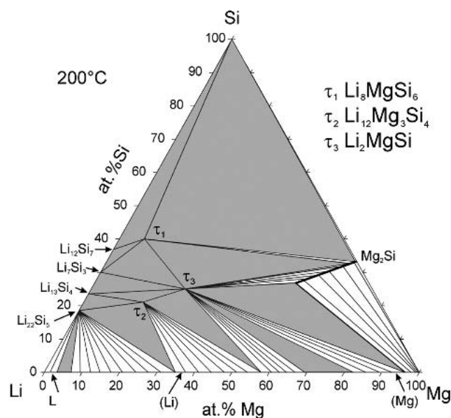
Fig. 22 Calculated isothermal section of Li-Mg-Si phase diagram at 200 °C
