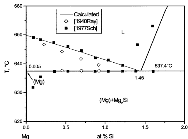
Fig. 6 Calculated Mg-rich side of the Mg-Si phase diagram (this work)
