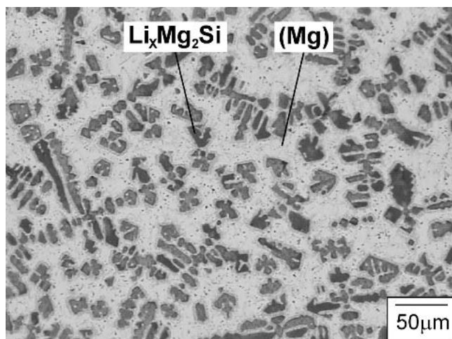
Fig. 17 Microstructure of Mg_{80}Li_{10}Si_{10} as-cast sample g after 20 h in dry air
