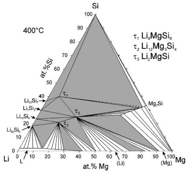
Fig. 21 Calculated isothermal section of Li-Mg-Si phase diagram at 400 °C
