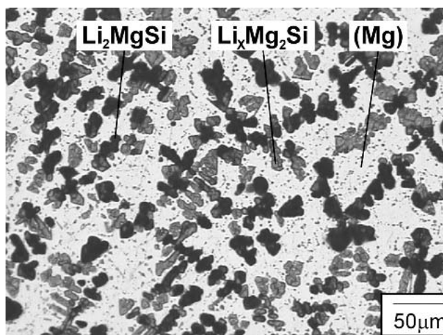
Fig. 18 Microstructure of Mg_{70}Li_{20}Si_{10} as-cast sample f after 20 h in dry air
