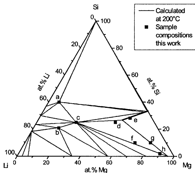
Fig. 10 Calculated isothermal section of the Li-Mg-Si phase diagram at 200 °C; details of the investigated samples are given in Table 1 and details of phase fields are given in Fig. 22.
