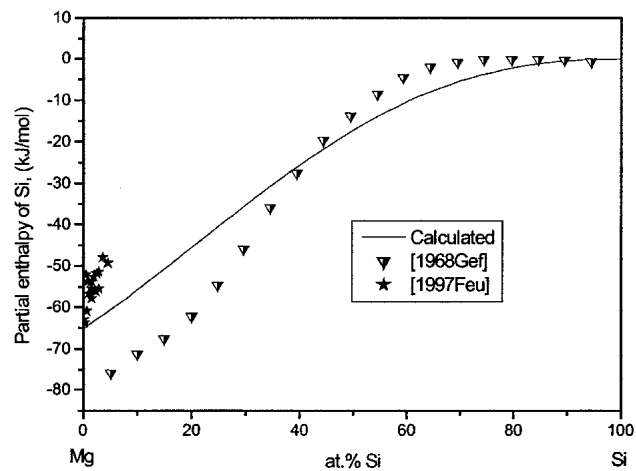
Fig. 9 Partial enthalpy of solution of Si in the liquid phase at 1077 °C (referred to Si l )
