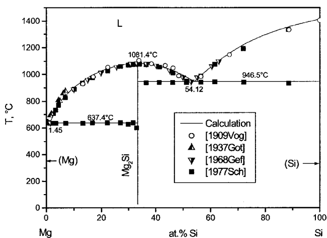
Fig. 5 Calculated phase diagram of the Mg-Si system (this work); the unrealistic inverted liquid miscibility gap at higher temperature does not occur, even if calculating beyond 4000 °C
