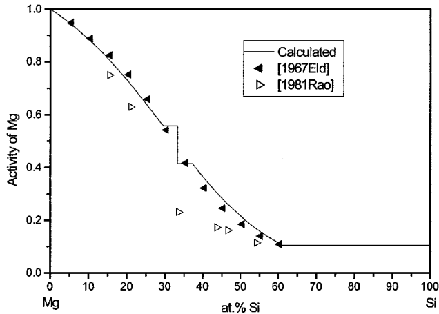
Fig. 7 Activity of Mg in liquid Mg-Si alloy at 1077 °C (referred to Mg l )
