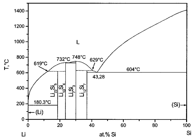
Fig. 2 Calculated phase diagram of the Li-Si system using parameters of [1995Bra]
