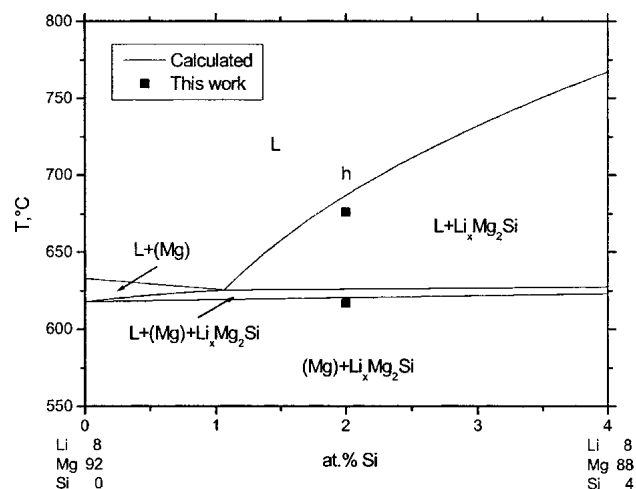
Fig. 16 Calculated partial polythermal section of the Li-Mg-Si system at 8 at.% Li compared with the DTA measurements for sample h
