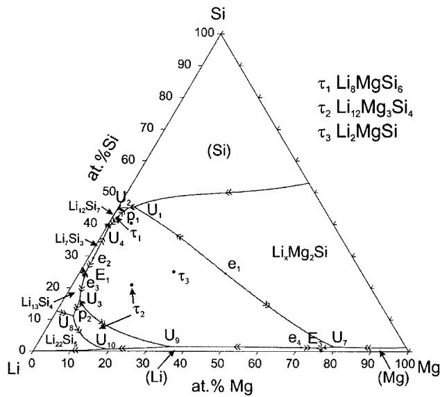
Fig. 19 Li-Mg-Si phase diagram, calculated liquidus surface; invariant reactions and fields of primary crystallization are marked.
