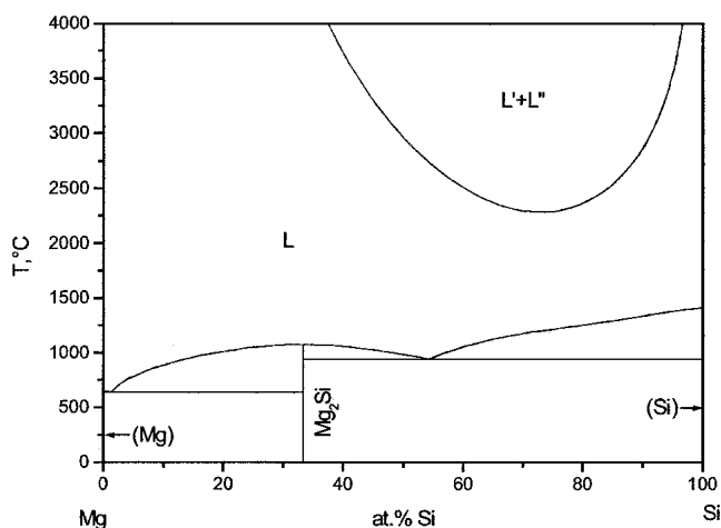
Fig. 3 Calculated phase diagram of the Mg-Si system using parameters of [1997Feu], producing an unrealistic liquid miscibility gap
