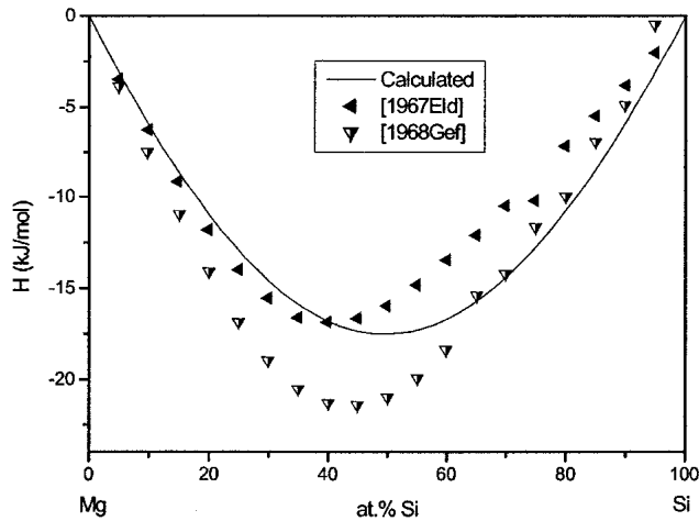
Fig. 8 Enthalpy of the liquid phase at 1077 °C (referred to Mg l and Si l )
