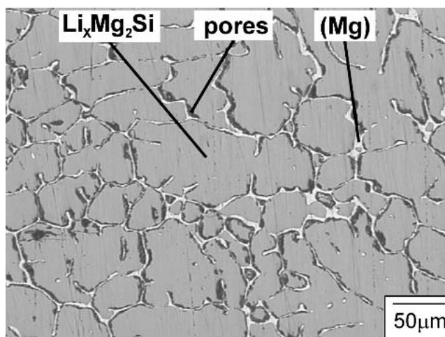
Fig. 11 Microstructure of the as-cast sample e with the composition \text{Li}_{14}\text{Mg}_{58}\text{Si}_{28} showing the \text{Li}_x\text{Mg}_2\text{Si} solid solution (gray) and small amount of Mg (light) in agreement with phase equilibria of Fig. 10
