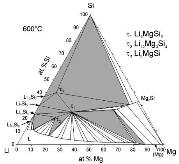
Fig. 20 Calculated isothermal section of Li-Mg-Si phase diagram at 600 °C
