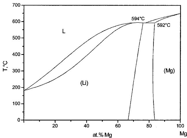
Fig. 1 Calculated phase diagram of the Li-Mg system using parameters of [1990Sau]
