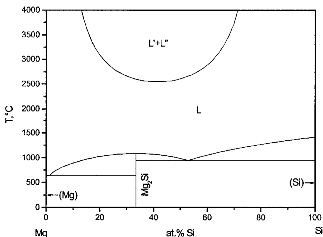
Fig. 4 Calculated phase diagram of the Mg-Si system using parameters of [2000Yan], producing an unrealistic liquid miscibility gap
